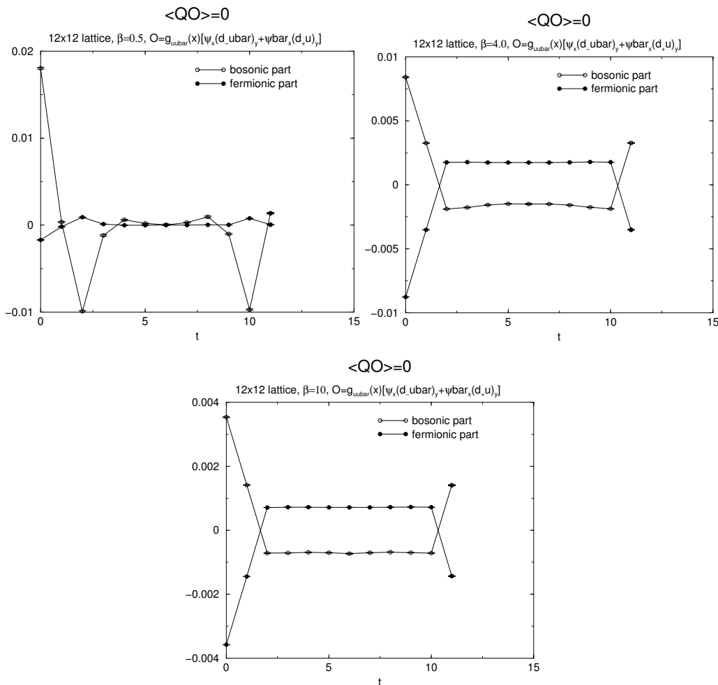
Figure 4: \langle QO \rangle = 0 for 12 \times 12 lattice
