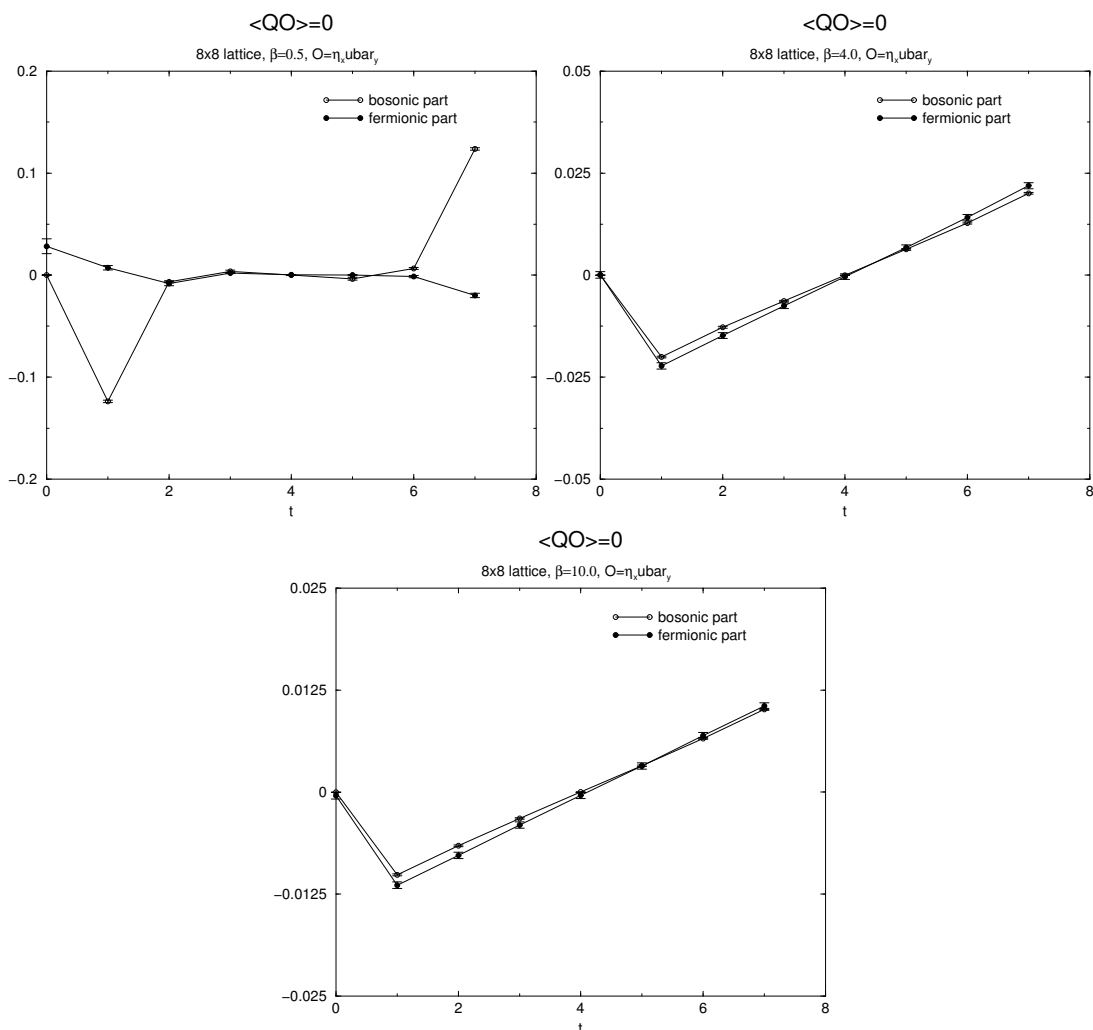
Figure 9: \langle Q(\eta_x \bar{u}_y) \rangle = 0 for 8 \times 8 lattice
