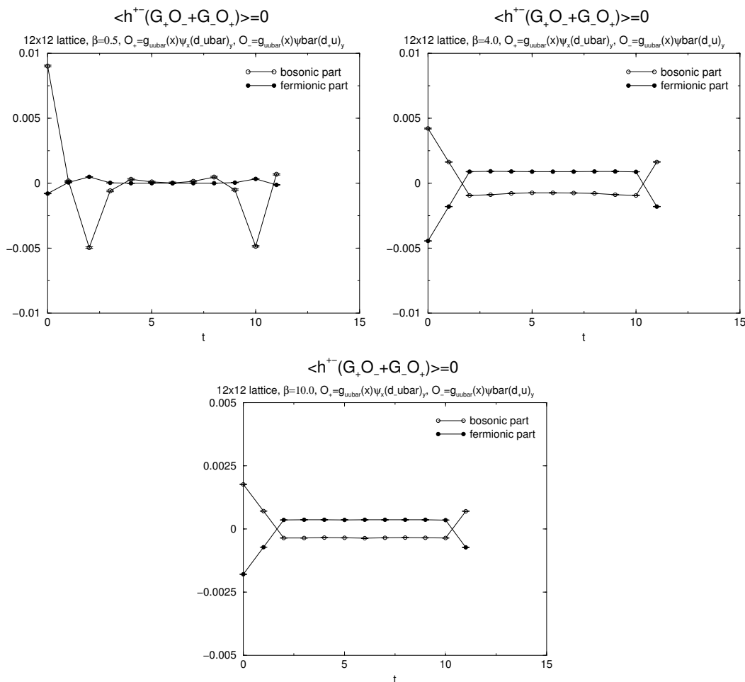
Figure 7: \langle h^{+-}(G_+O_- + G_-O_+) \rangle = 0 for 12 \times 12 lattice
