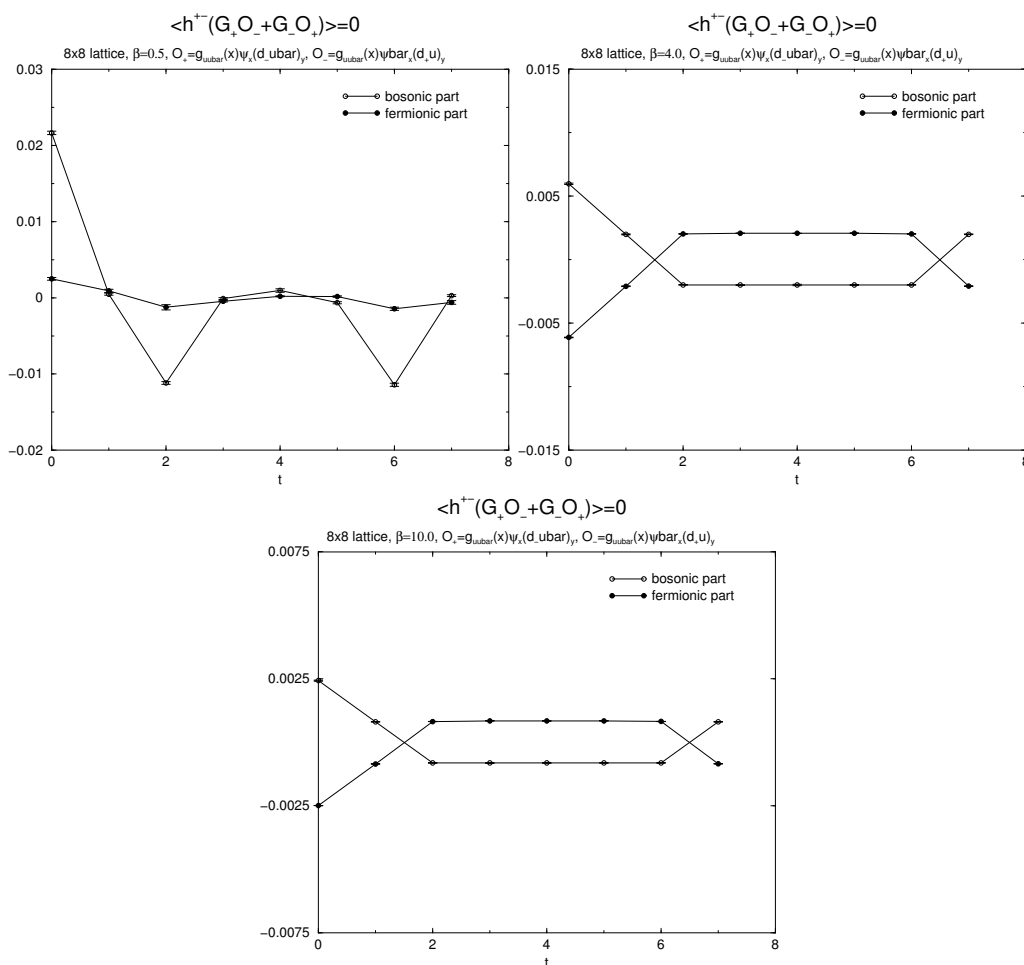
Figure 6: \langle h^{+-}(G_+O_- + G_-O_+) \rangle = 0 for 8 \times 8 lattice
