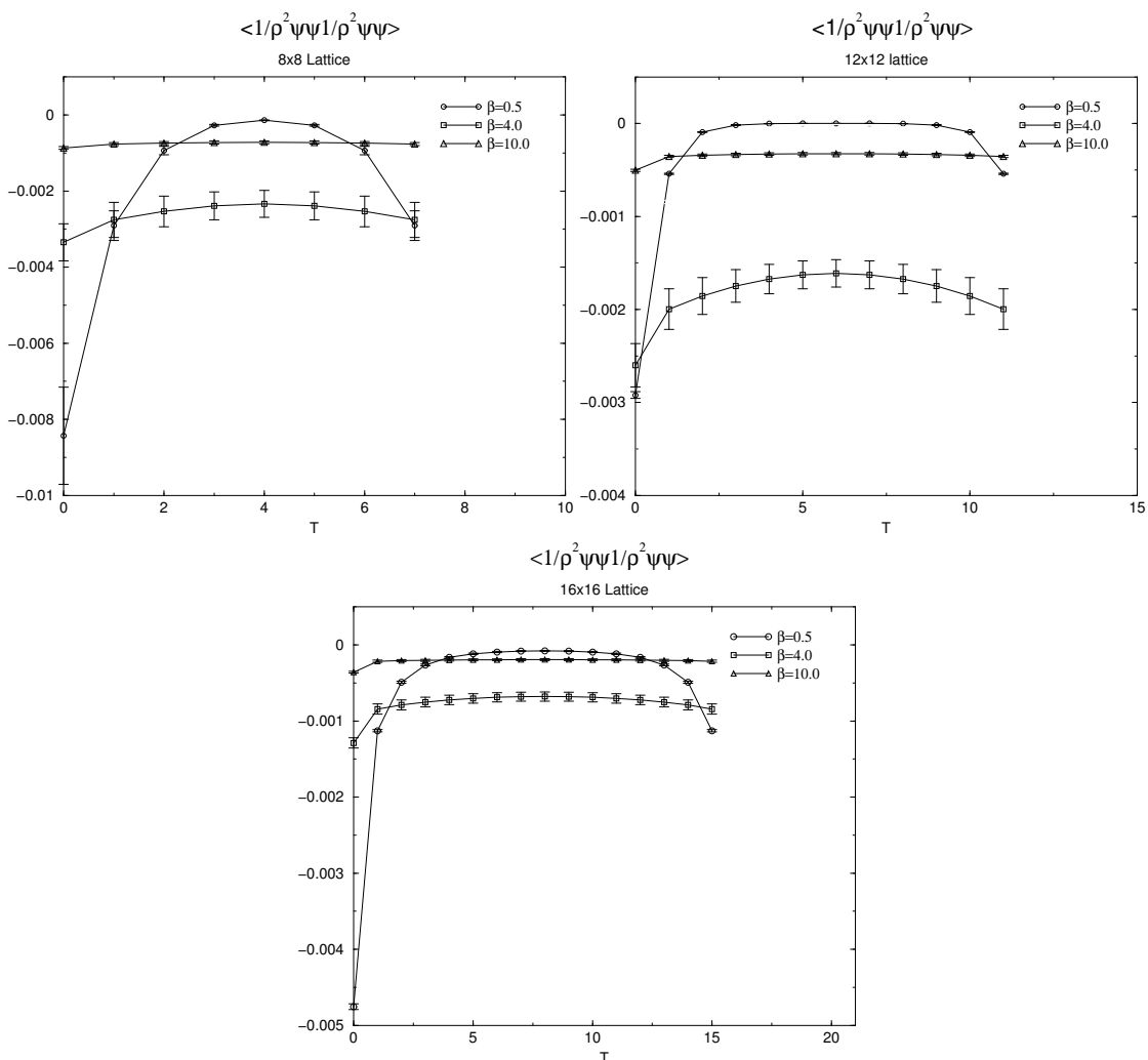
Figure 10: Condensate for 8x8, 12x12 and 16x16 lattices
