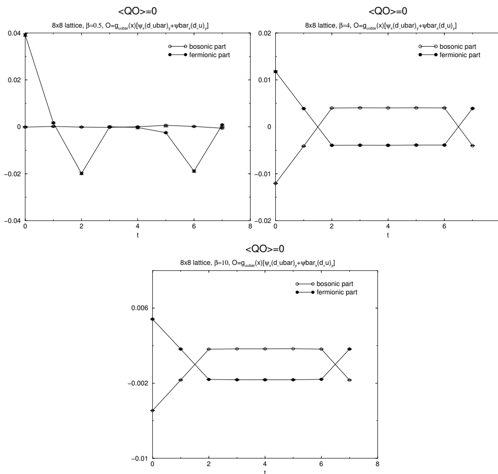
Figure 3: \langle QO \rangle = 0 for 8 \times 8 lattice
