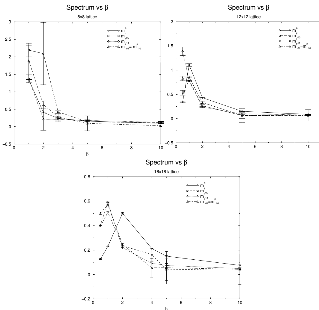
Figure 1: Mass spectrum for 8x8, 12x12 and 16x16 lattices
