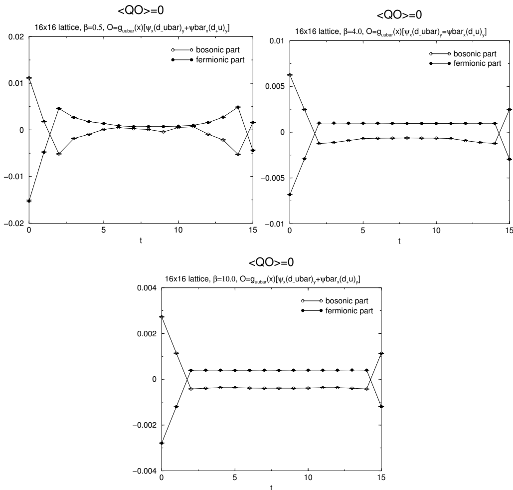
Figure 5: \langle QO \rangle = 0 for 16 \times 16 lattice
