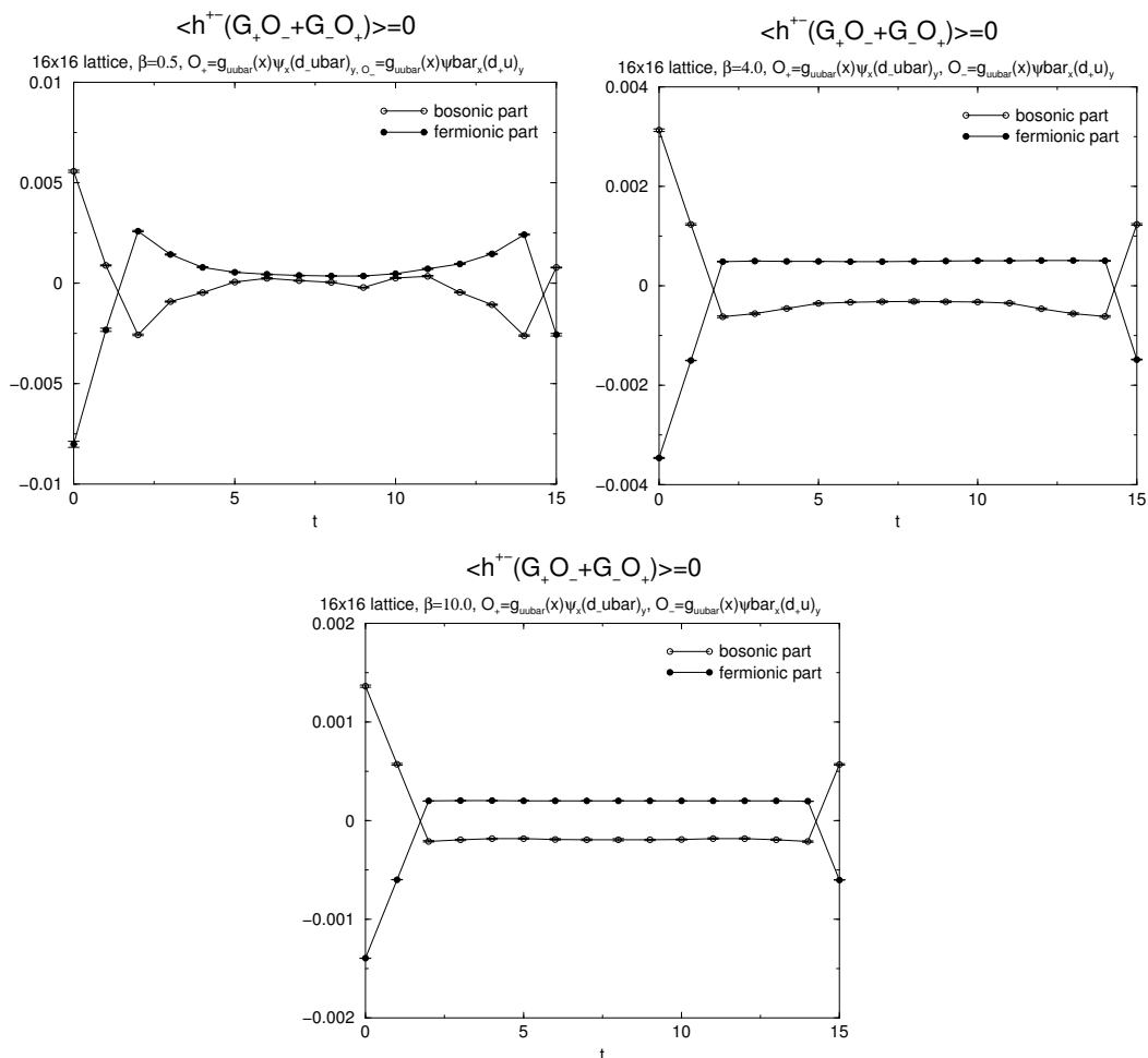
Figure 8: \langle h^{+-}(G_+O_- + G_-O_+) \rangle = 0 for 16 \times 16 lattice
